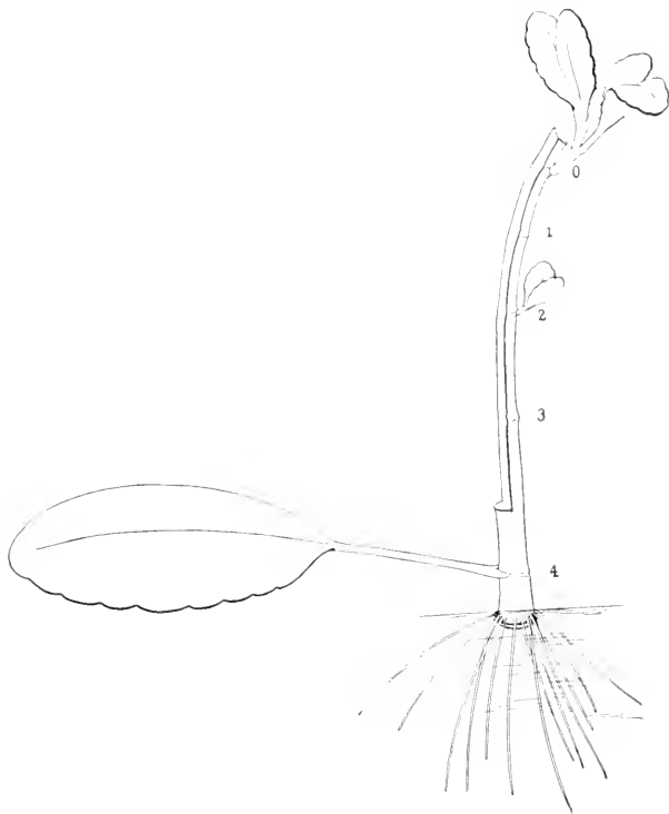
FIG. 97.—Half stem with leaf at base. Nov. 12 to Dec. 5, 1923.
